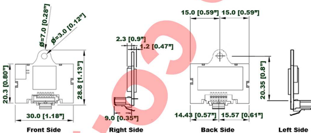
Horizontal Type Low Profile with mounting hole Micro SATA Flash Module
