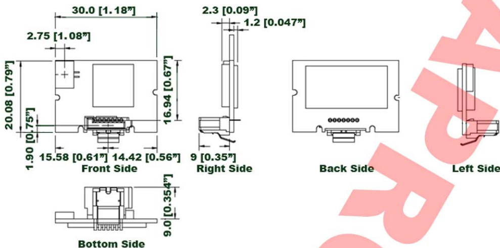
Horizontal Type Low Profile Micro SATA Flash Module
